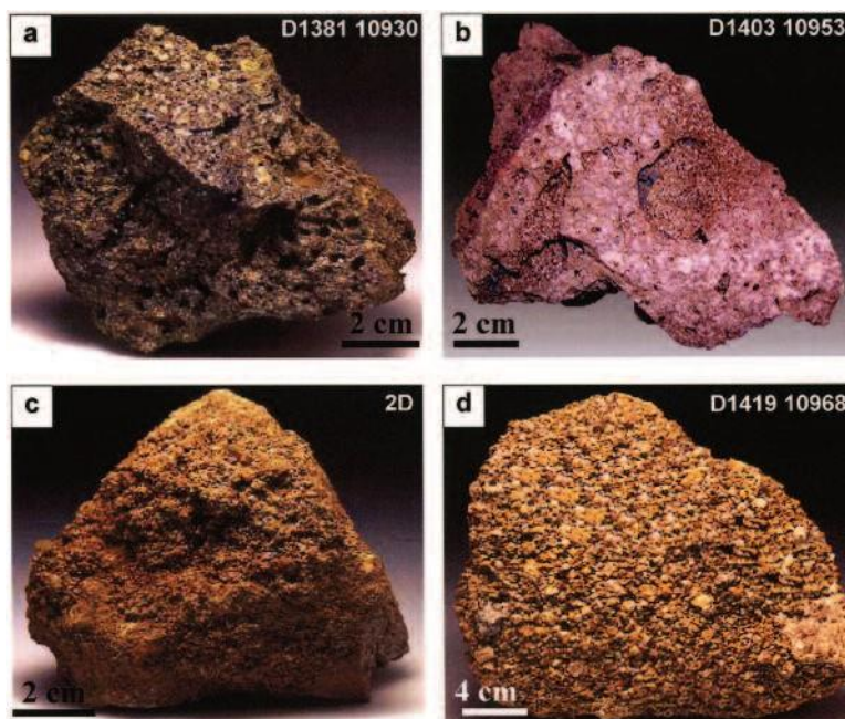
Fig. 2 - selected lithologies from 1872 eruption: (a) hI, (b) Cl, (c) ImC, (d) C (see table 1 for label explanation).
