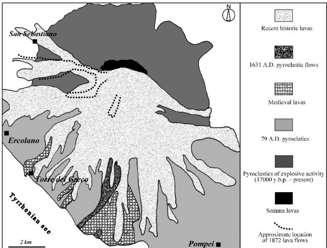
Fig. 1 - schematic geo-volcanological map of somma-Vesuvius (redrawn after ayuso et al. , 1998).
