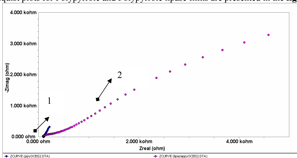
Figure 3 The Niquist curves of Polypyrrole (1) and Polipyrrole with lipase (2) films in 0,5 M \text{Na}_2\text{SO}_4 solution obtained between 100 KHz and 0,01Hz frequencies
