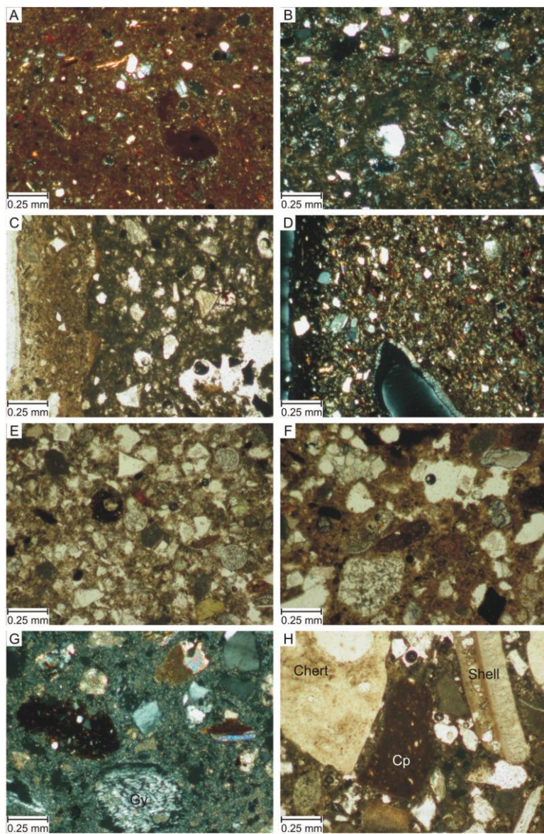
Fig. 4 – optical photomicrographs (polarized light) of bricks and mortars. a) red brick with quartz-feldspar-phyllsilicates plus cocchiopesto frame in a fine-grained reddish groundmass with scattered vacuoles (sample It1 , nX); B) yellow brick with quartz-feldspar sandy frame in brown vacuolar groundmass ( It2 , nX); c) yellow brick showing a thin layer of lime plaster (“ sagramatura ”, left) ( It3 , n//); D) rose brick rich of quartz-feldspar fragments and macropores with calcite rims and a thin lime plaster (left) ( It6 , nX); e) lime bedding mortar, sand frame with scattered foraminifers shells and cocchiopesto (M7, n//); F) Finishing plaster mortar, similar to 4e (M4, n//); G) Finishing plaster mortar with crystalline gypsum (Gy) fragment (M8, nX); h) Micro-conglomeratic plaster mortar with chert, cocchiopesto (Cp) and shells fragments (M1, n//).
