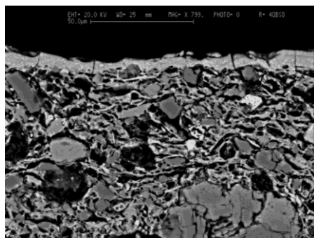
Fig. 7 – SEM backscattering electron microphotograph of gloss pottery; sample 207. gloss thickness is 29 \mu\text{m} in this area.
